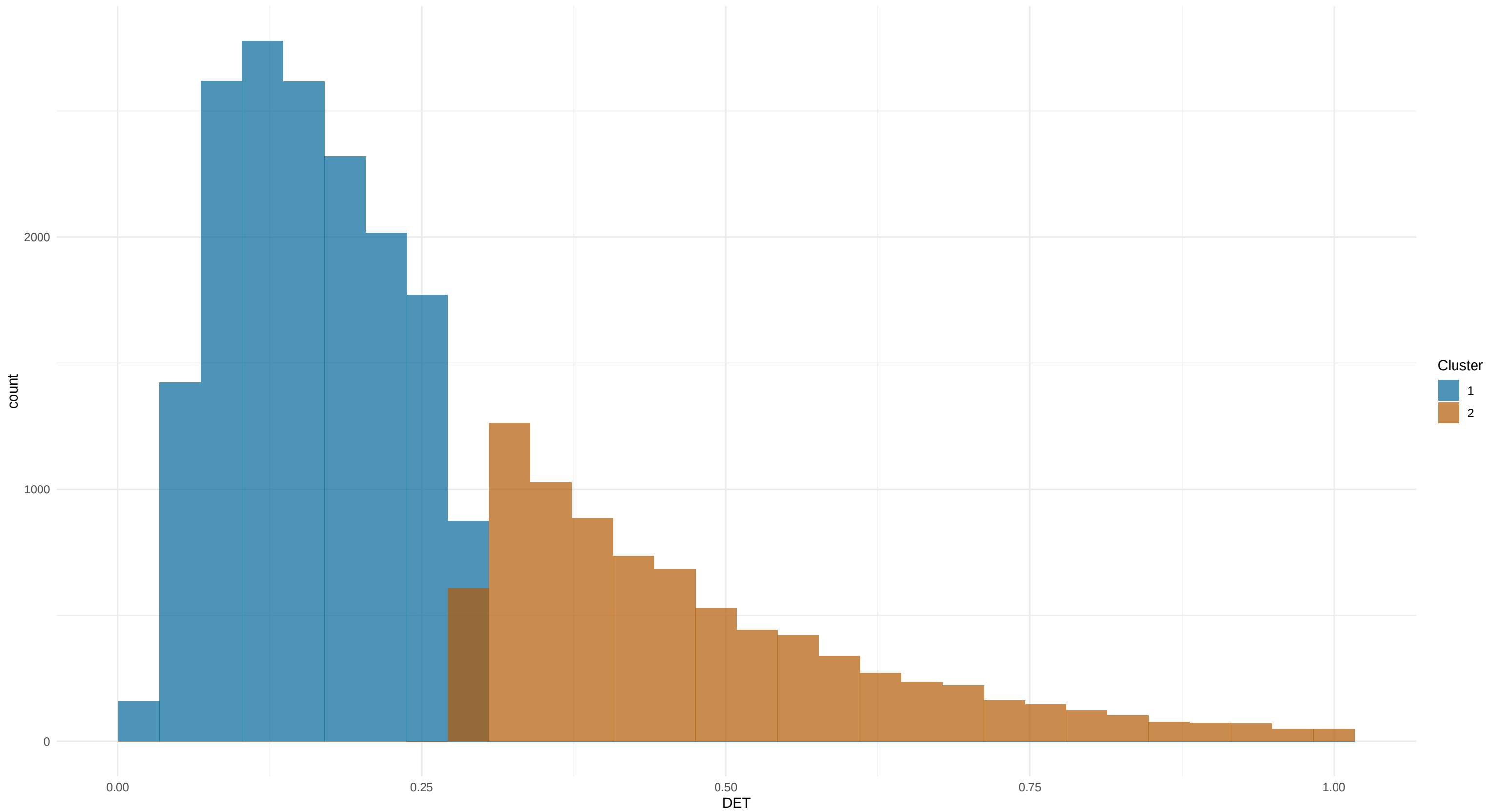
DET clustered into automatic groups
